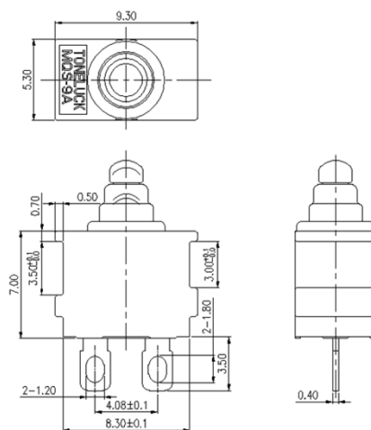
Location Pin(Type E)、Terminal(TypeF)
