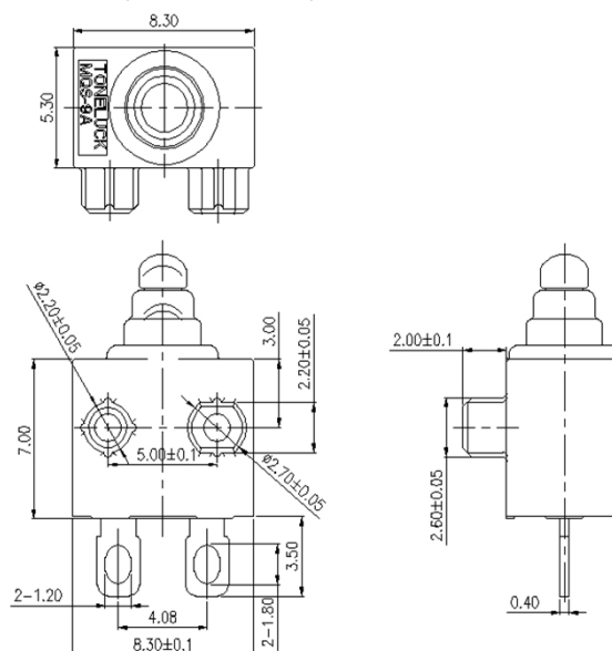
Location Pin(Type F)、Terminal(TypeD)
